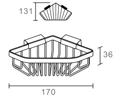
# 030509 Eckseifenkörbchen Messing, verchromt Corner Soap Basket Brass, chrome finish
