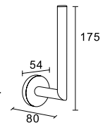
# 710009 Reserverollenhalter Spare Roll Holder
