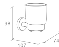
740052 Glashalter Satinieretes Glas / Glass Holder Iced Glass
